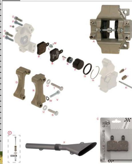
Tav. 33 PINZA FRENO POSTERIORE • REAR BRAKE CALIPER BS6
